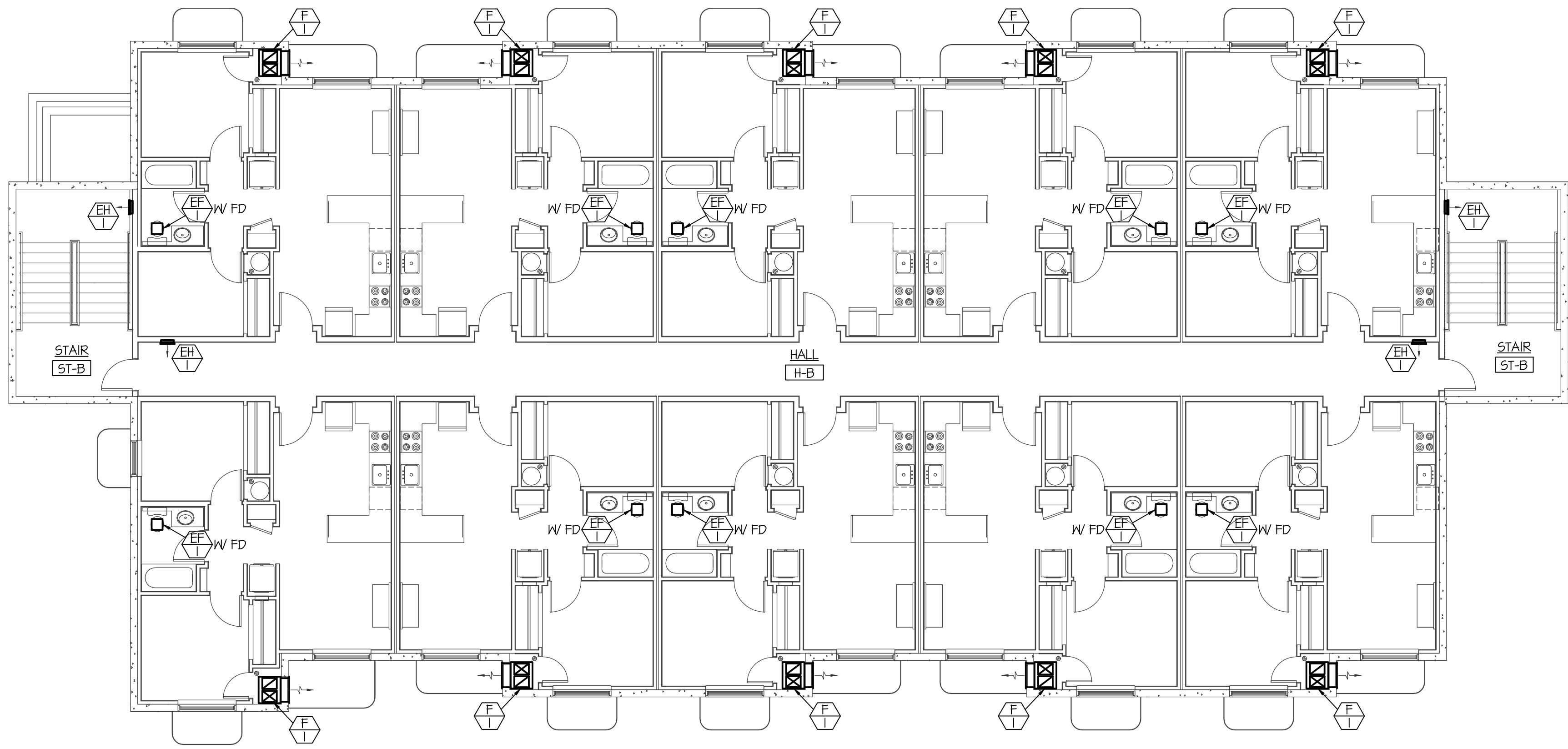
BLDG. 1 BASEMENT MECH. FLOOR PLAN SCALE: 1/8" = 1'-0"
