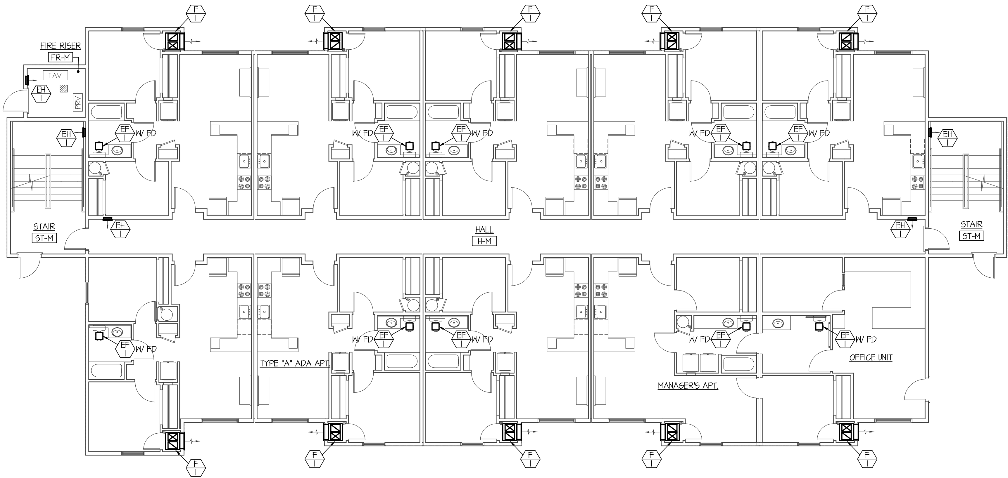
BLDG. 1 MAIN FLOOR MECH. PLAN SCALE: 1/8" = 1'-0"
